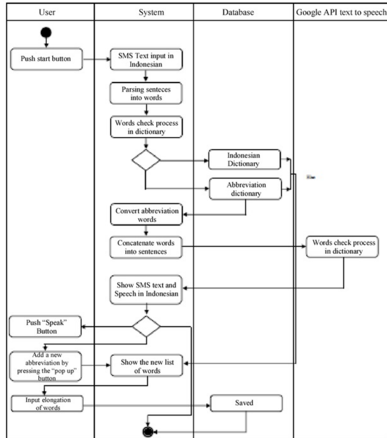
Fig. 2: Diagram activity text to speech for abbreviation in SMS text (Areni et al. , 2017a)
