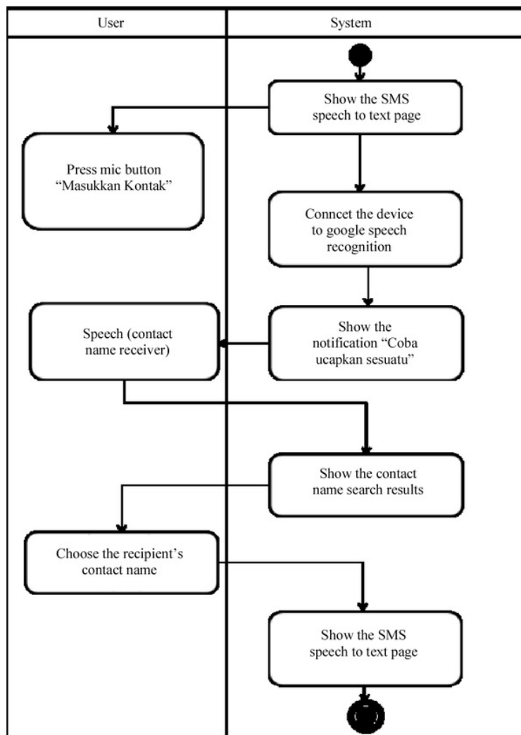
Fig. 4: Activity diagram for speech to add contact
